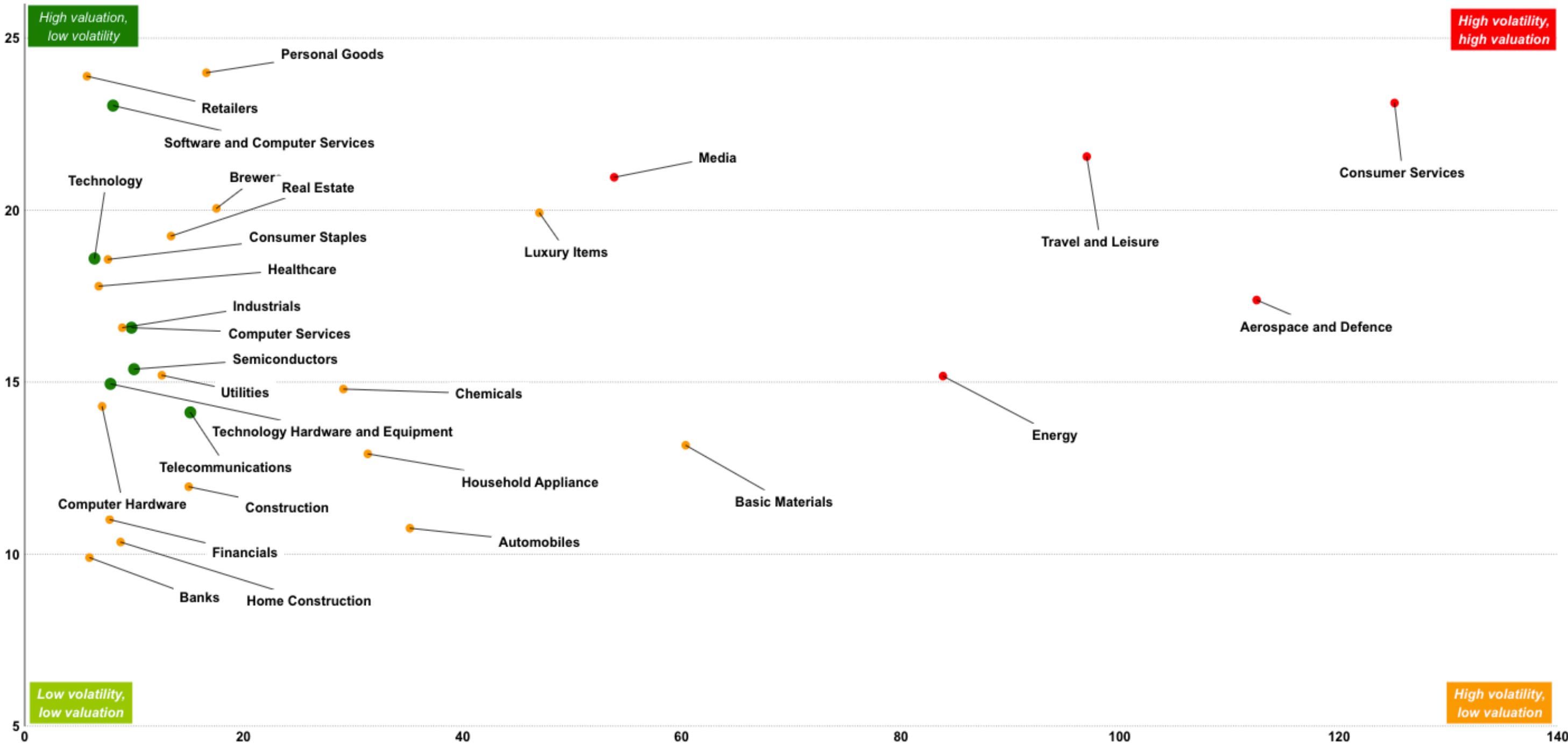
Forward P/E ratio and earnings growth volatility
